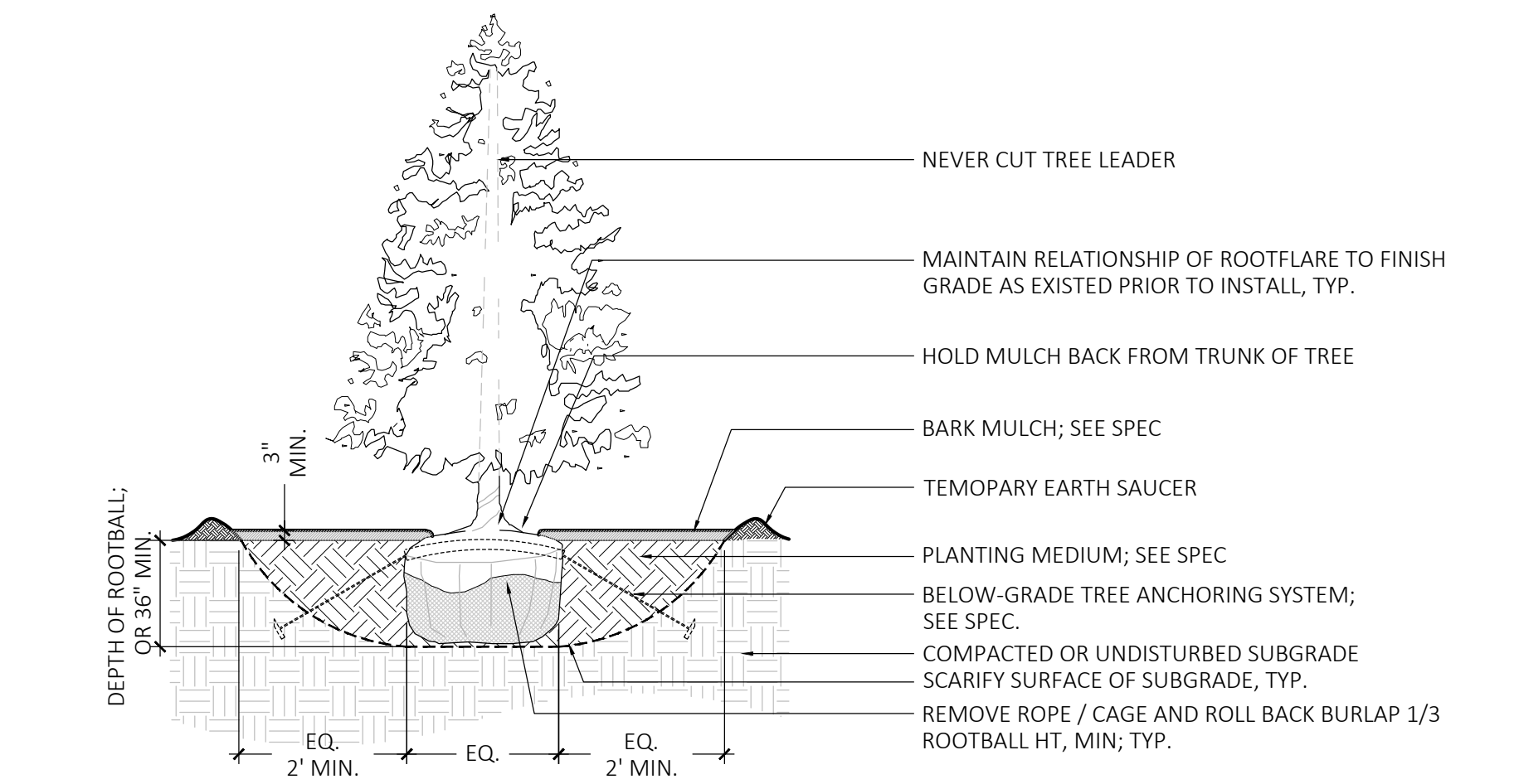
5 EVERGREEN TREE PLANTING NOT TO SCALE
